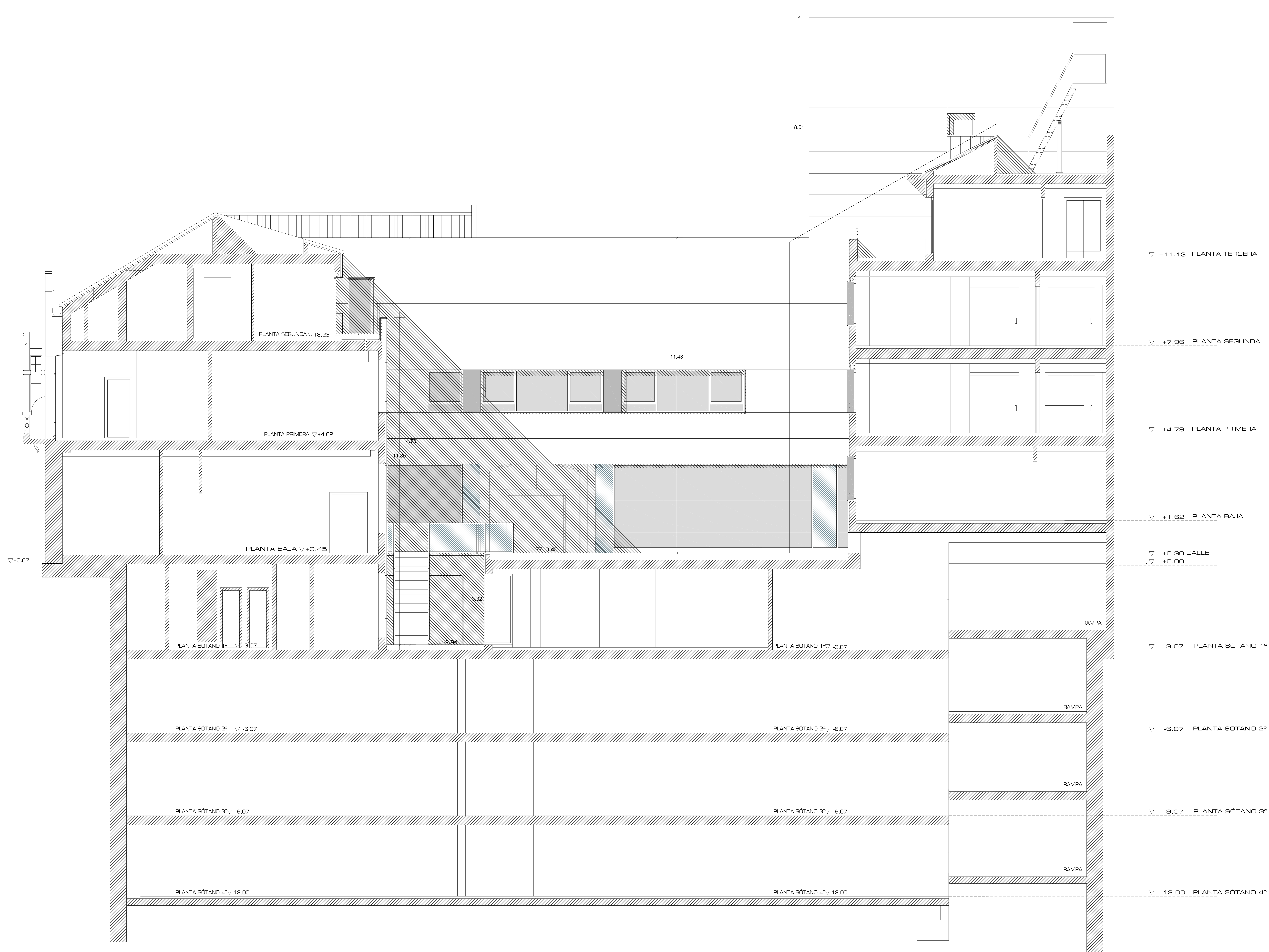
ALZADO INTERIOR B
